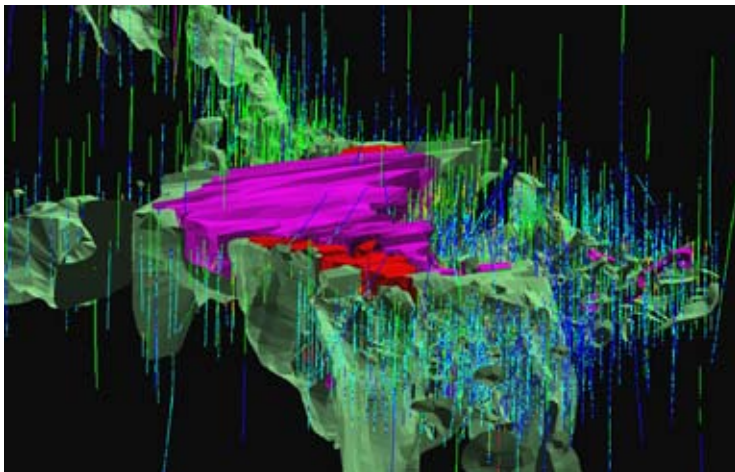
Geological interpretation from ODX resource drilling
