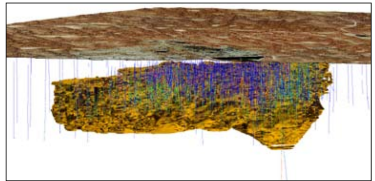
Cu grade shell of Olympic Dam deposit compared to resource
